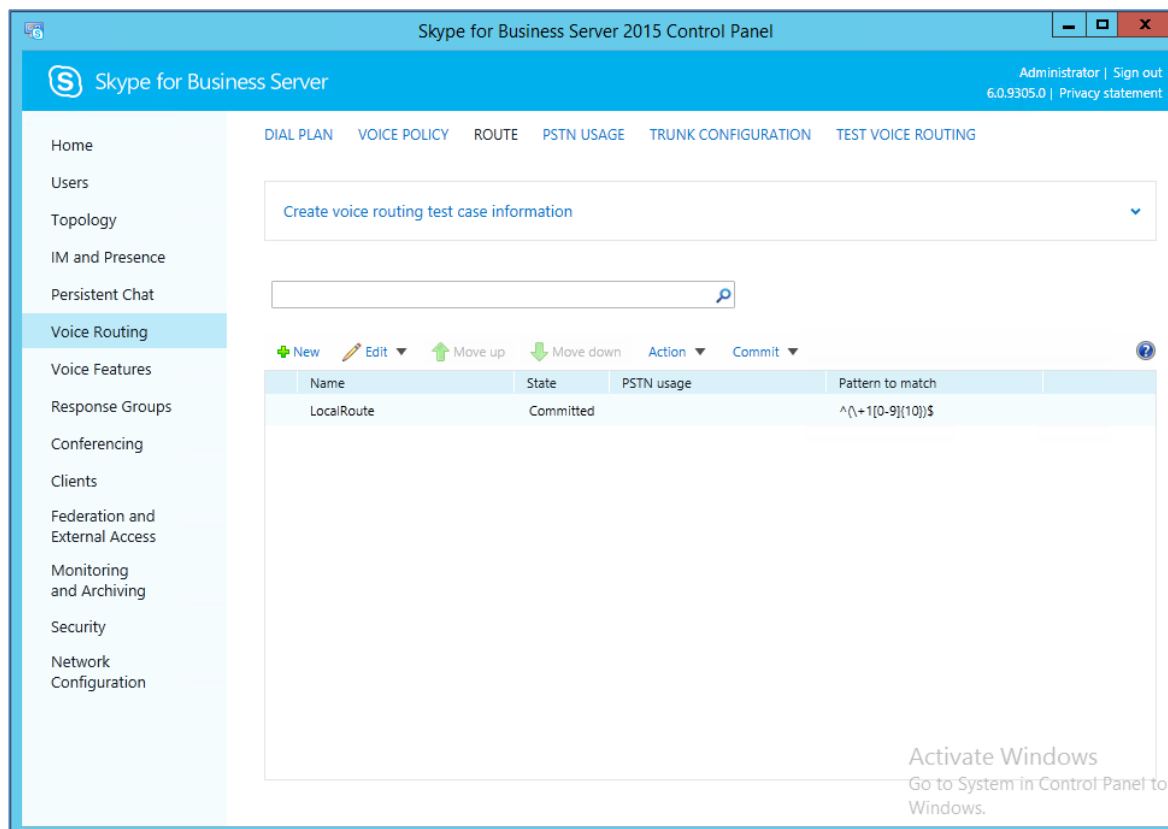
Figure 3-18: Route Tab
